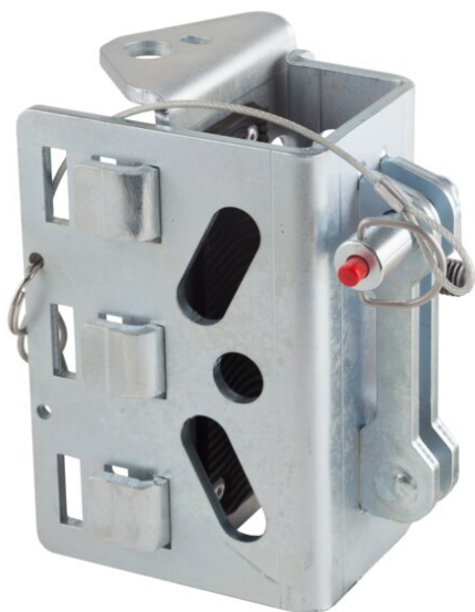
UTB mounting on a tripod leg
