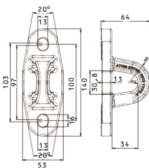
Figure 2. Overall dimensions AT150
