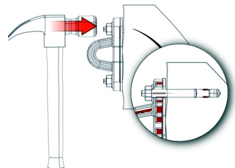
Figure 10. Embedding throughbolts in concrete.
